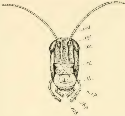
FIG. 17.—Front-view face of grasshopper ( Schizocerca americana ): ant. , antenna; oc. , ocellus; eye. , eye; cl. , clypeus; lbr. , labrum, or upper lip; mx.p. , maxillary palpus; lab.p. , labial palpus; gal. , galea, lobe of maxilla; lab. , labium, or under lip.
